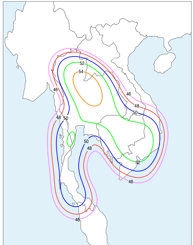
Downlink Contour
